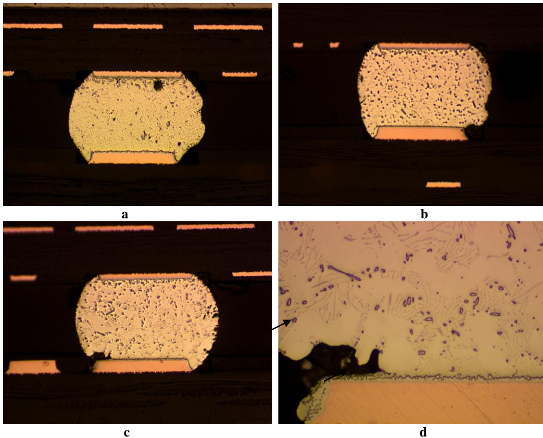
Figure 14. Defects of Mirrored \mu\text{BGAs} after Topside Rework: a, b, c – 100\times ; d – 400\times
