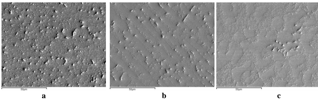
Figure 11. Microstructure of a Centre Ball from a Primary Attached \mu BGA (a), a Reworked \mu BGA
